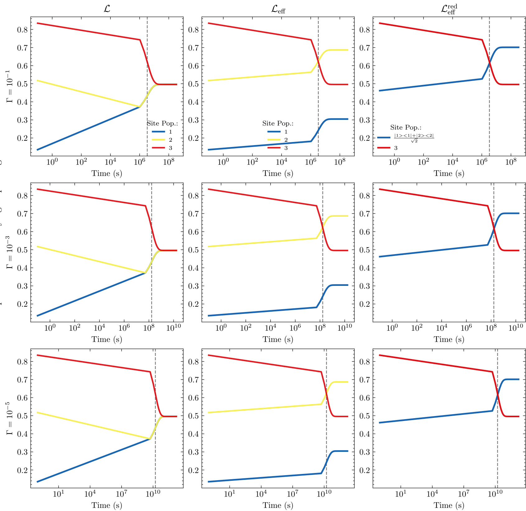
Time Evolution of Site Populations under \mathcal{L} , \mathcal{L}_{\text{eff}} , and \mathcal{L}_{\text{eff}}^{\text{red}} N=3 ; N_{\text{dimers}}=1 ; N_{\epsilon}=1 ; J = 10^{-1} ; \epsilon = 10^{-4} ; seed=722
